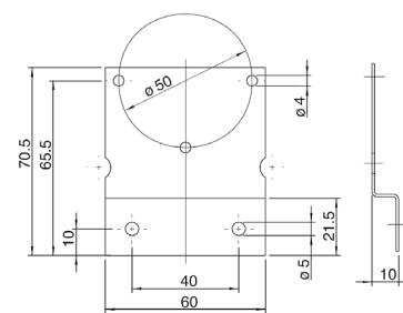
Mounting bracket 6402
