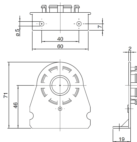
Mounting bracket 6482
