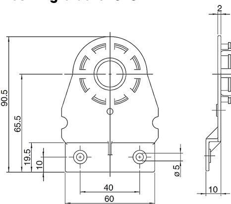
Mounting bracket 6482
